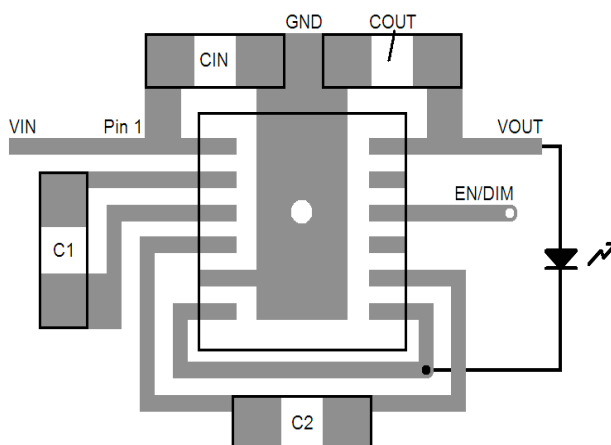
Figure 29. Recommended Layout
